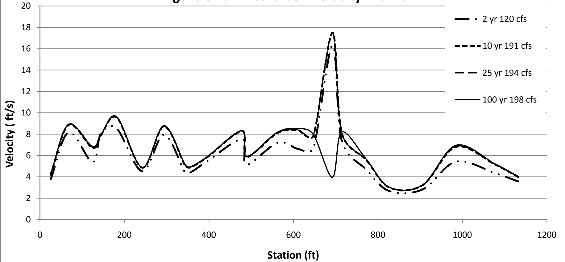
Figure 5. Chimes Creek Velocity Profile
